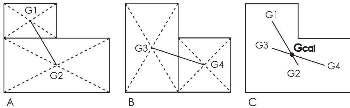
Fig. 3 The projection of the center-of-gravity of the L-shaped plane is calculated from the position of the center-of-gravity of rectangles that constitute the shape. G1, G2, G3 and G4 are the center-of-gravity of each rectangle. Gcal is the center-of-gravity of the L-shape plane.
