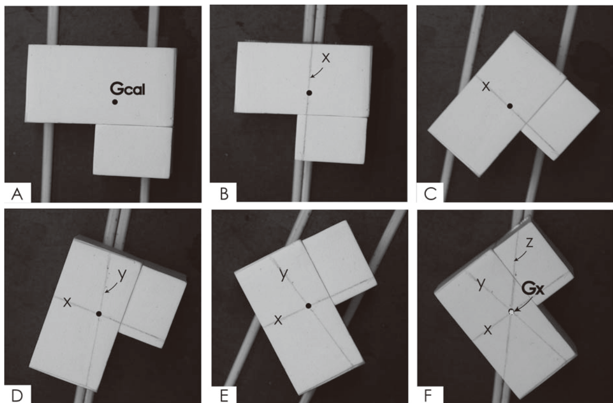
Fig. 4 The projection of the center-of-gravity of the L-shaped plaster object was determined ( Gx ). Gcal is the predicted position of the center-of-gravity required in calculation as shown in Fig. 3. Adjoined two sticks on the balanced line (x, y and z) where the projection should be situated. The intersection of the three balance lines is the projection of the center-of-gravity on the L-shaped plane ( Gx ). The position of Gx and Gcal coincides with each other.
